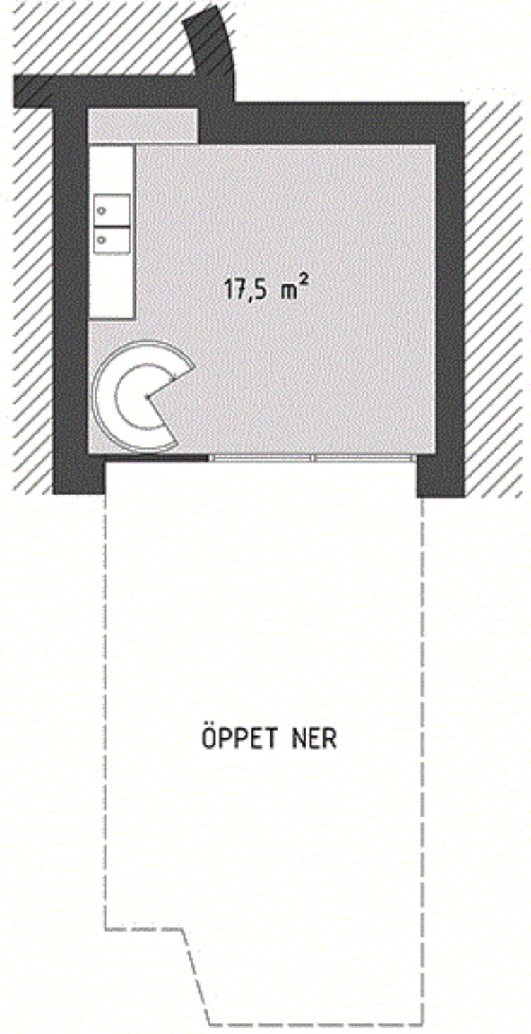
PLAN 2
