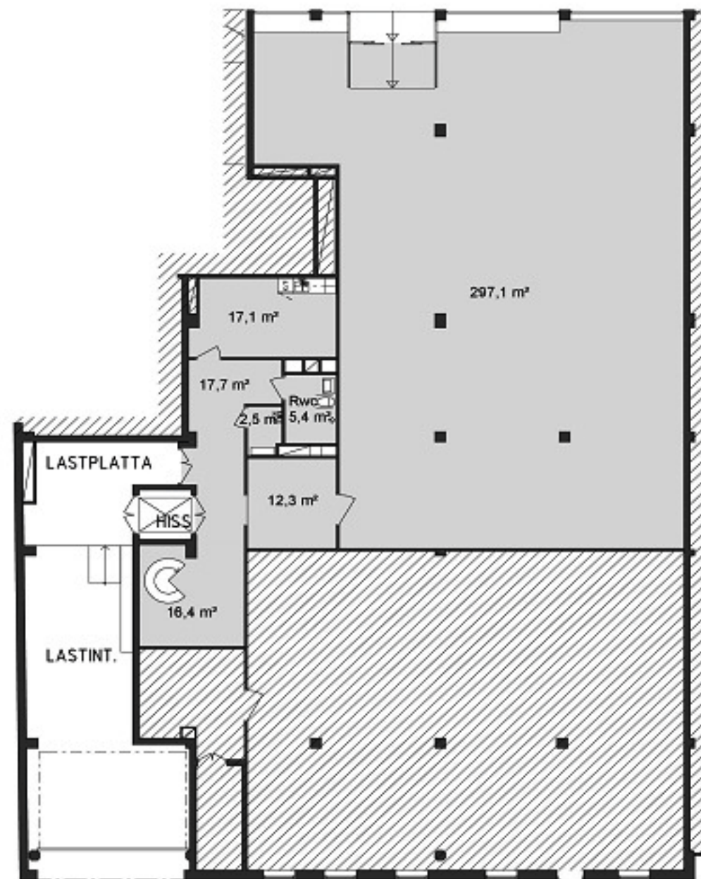
BOTTENPLAN
