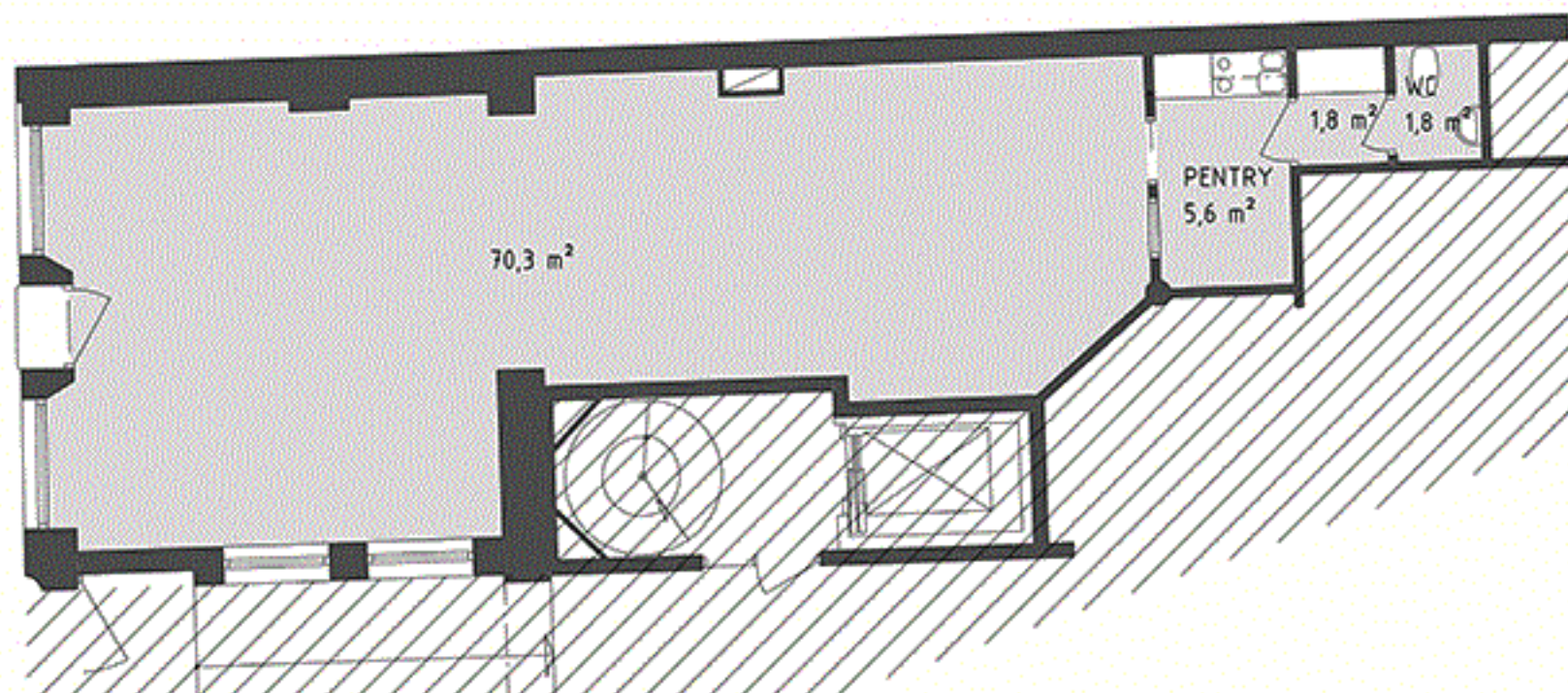
BOTTENAPLAN
